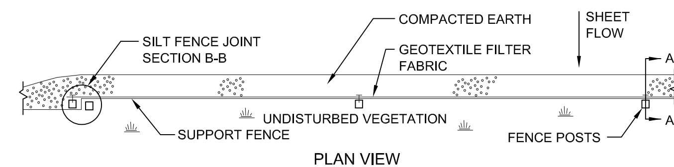
PLAN VIEW
