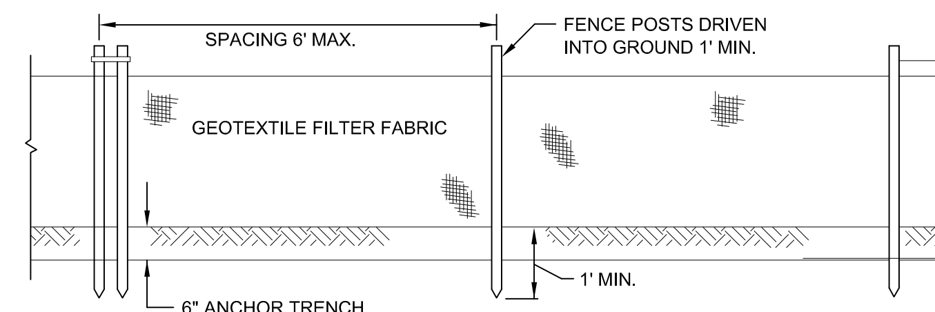
FRONT VIEW
