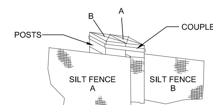
SECTION B-B JOINT
